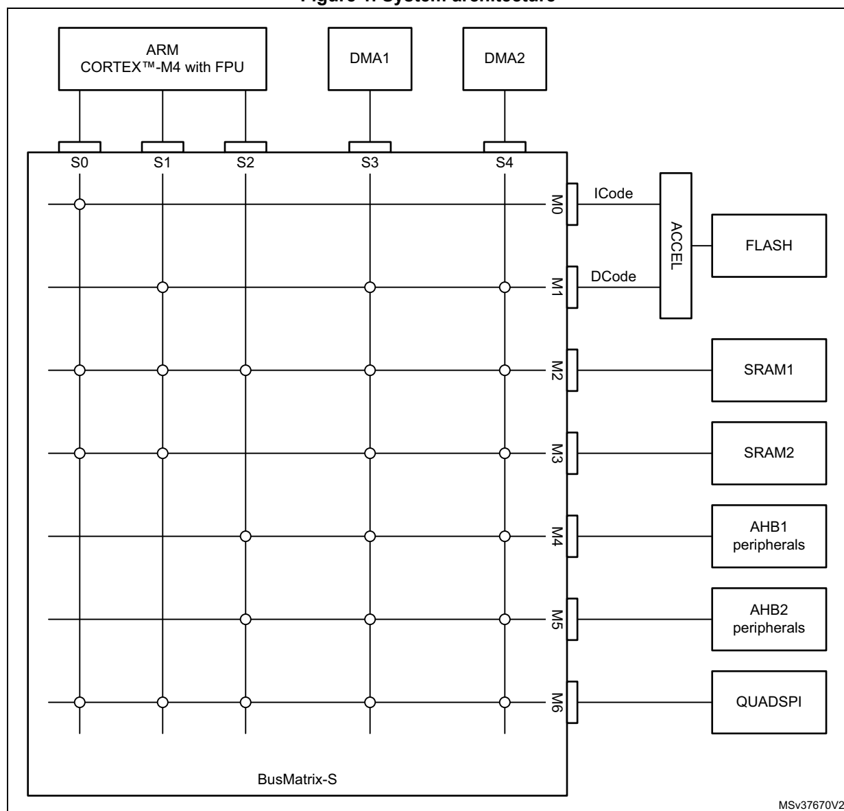
Figure 1. System architecture
