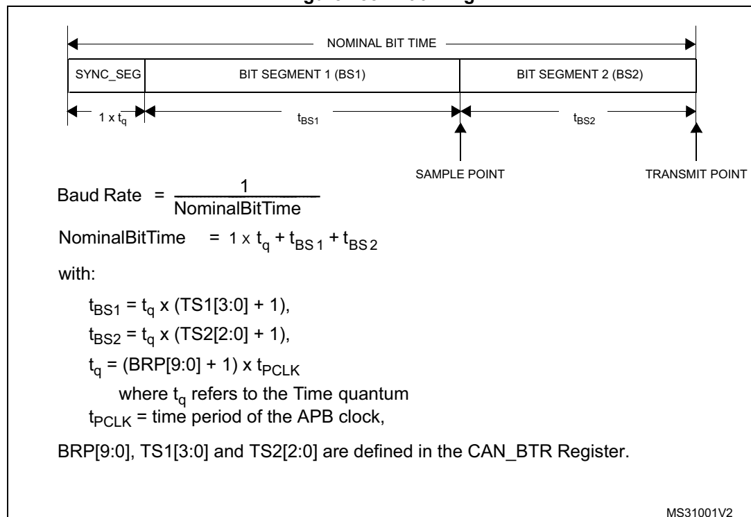
Figure 488. Bit timing
