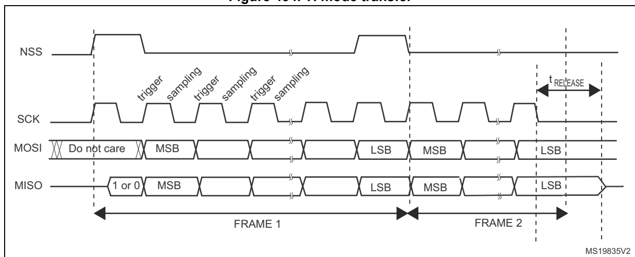
Figure 434. TI mode transfer
