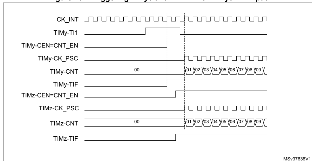
Figure 291. Triggering TIMy3 and TIMz2 with TIMy3 TI1 input
