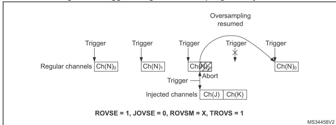
Figure 88. Triggered regular oversampling with injection
