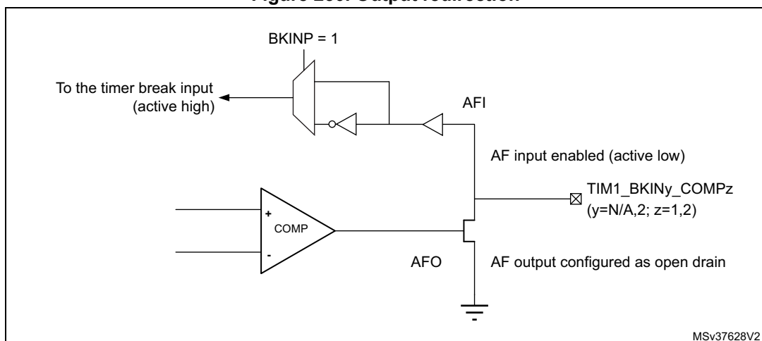
Figure 230. Output redirection
