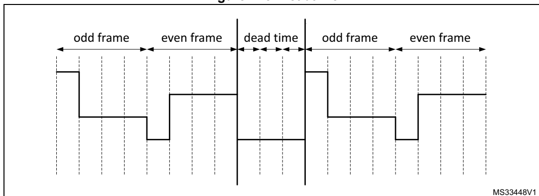
Figure 143. Deadtime
