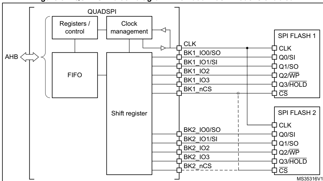
Figure 32. QUADSPI block diagram when dual-flash mode is enabled
