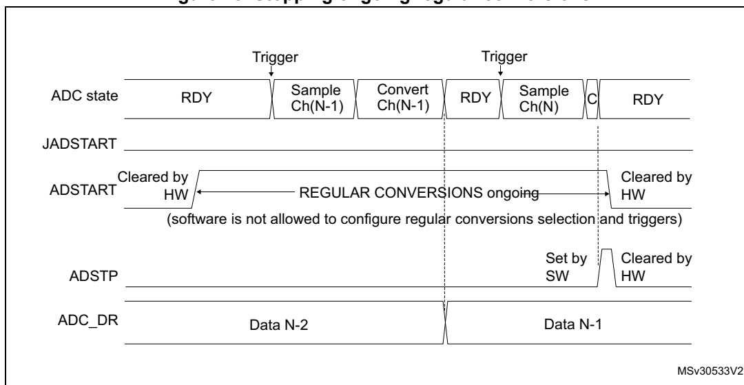
Figure 48. Stopping ongoing regular conversions
