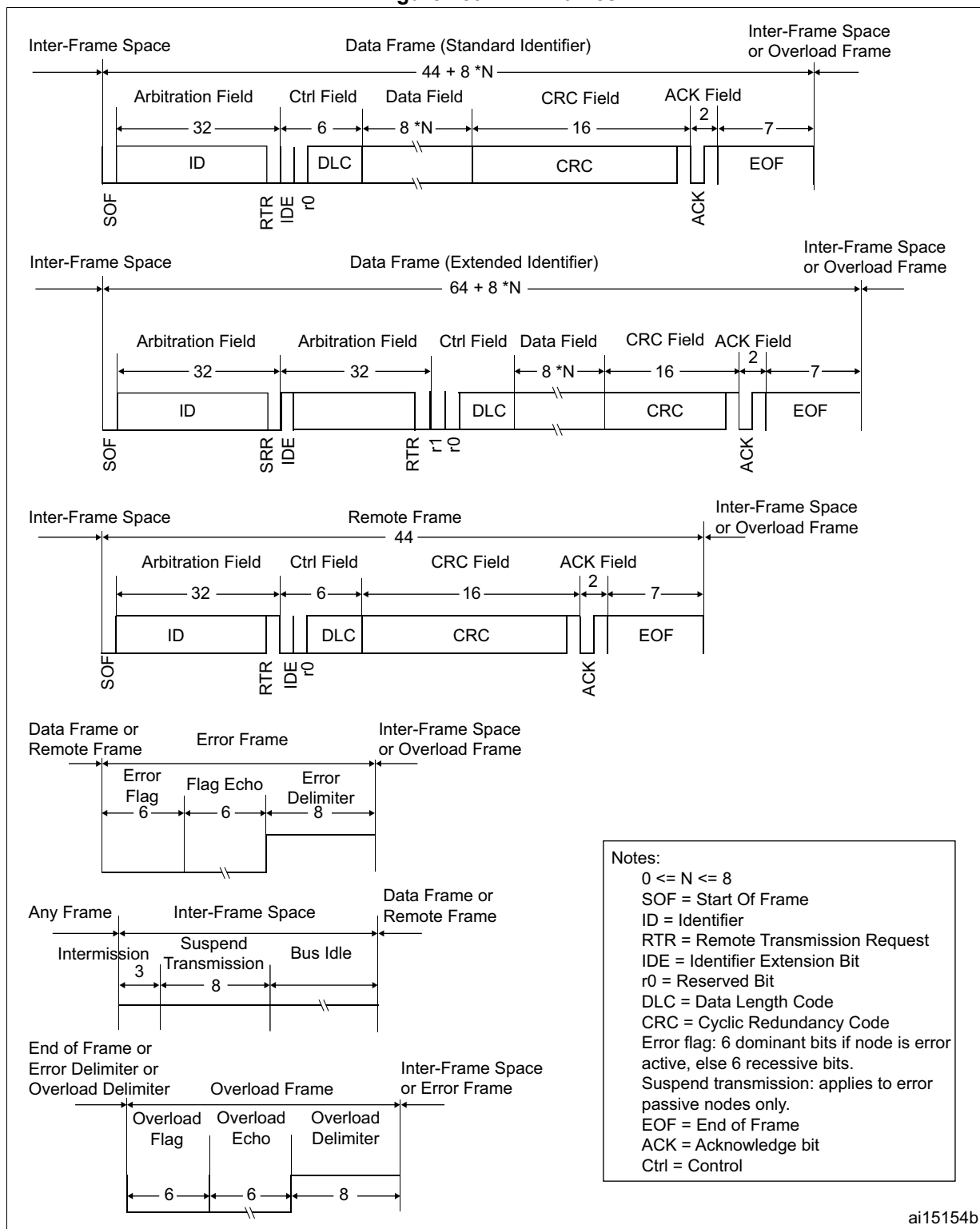
Figure 489. CAN frames
