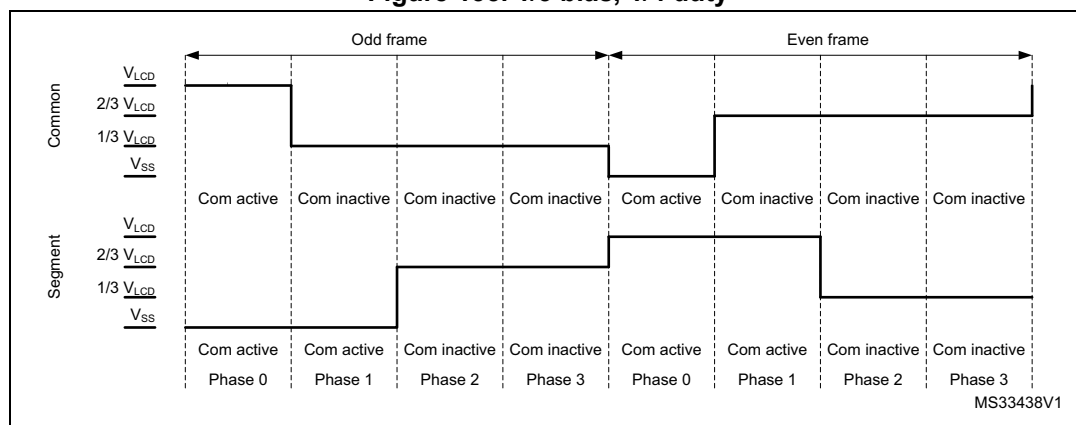
Figure 135. 1/3 bias, 1/4 duty
