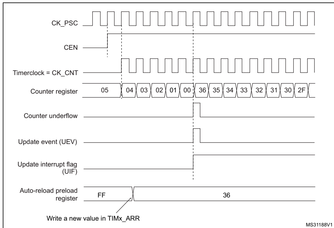
Figure 256. Counter timing diagram, Update event when repetition counter is not used
