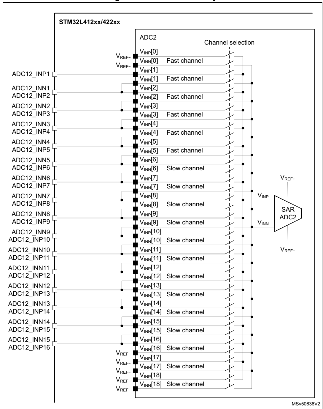
Figure 42. ADC2 connectivity
