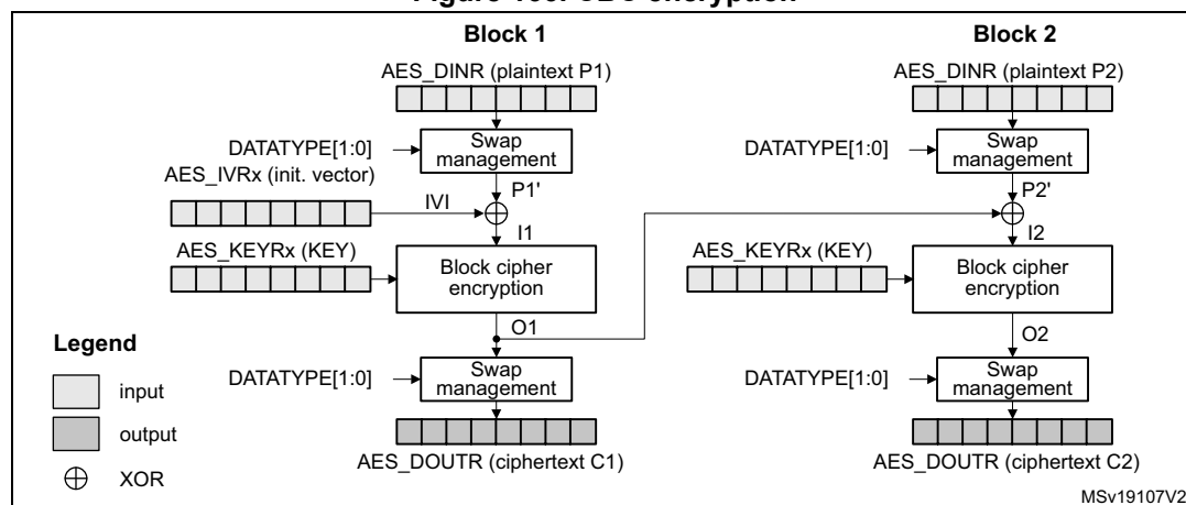
Figure 166. CBC encryption
