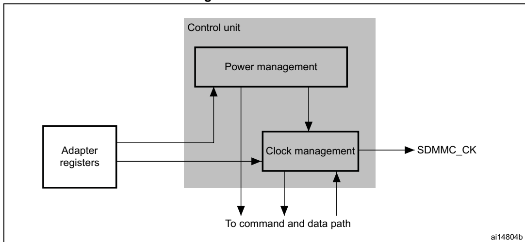
Figure 469. Control unit
