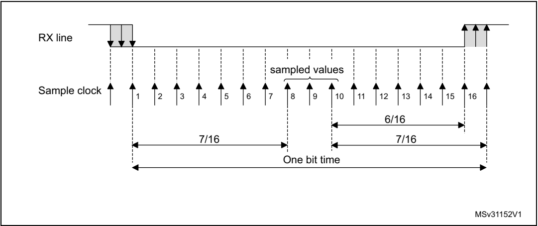
Figure 387. Data sampling when oversampling by 16
