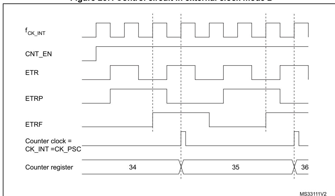
Figure 267. Control circuit in external clock mode 2
