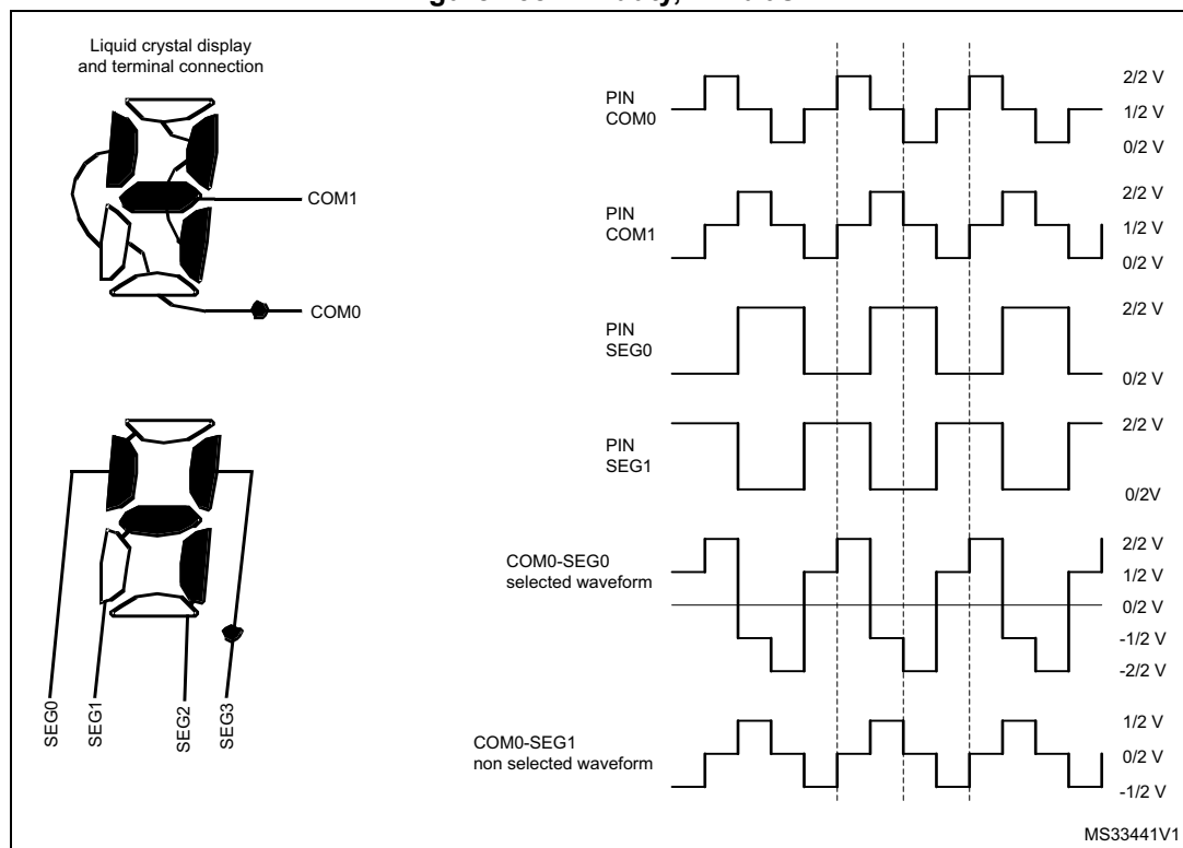
Figure 138. 1/2 duty, 1/2 bias
