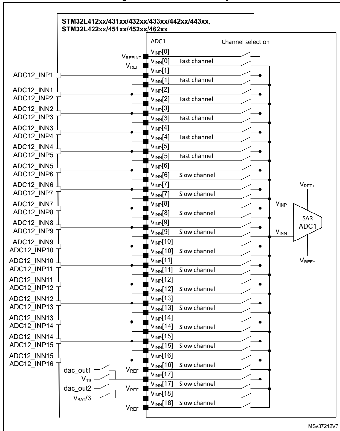
Figure 41. ADC1 connectivity
