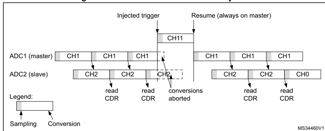
Figure 95. Interleaved conversion with injection
