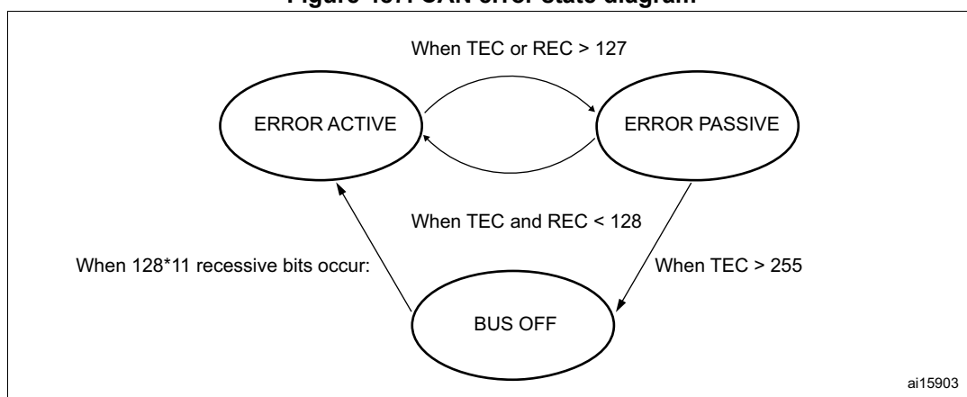
Figure 487. CAN error state diagram
