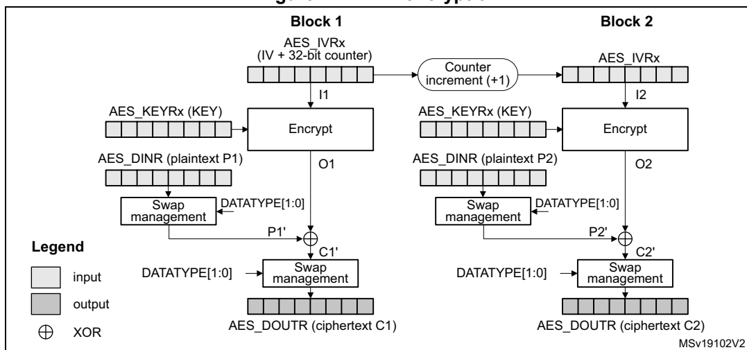
Figure 171. CTR encryption
