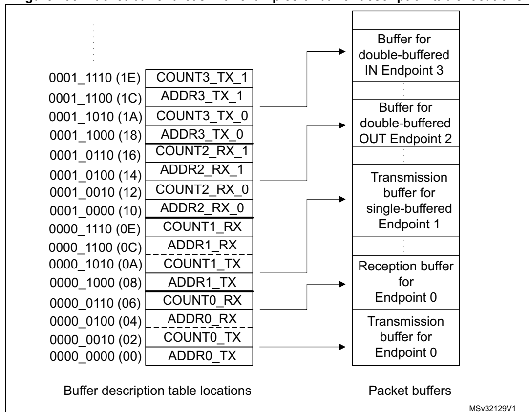
Figure 493. Packet buffer areas with examples of buffer description table locations
