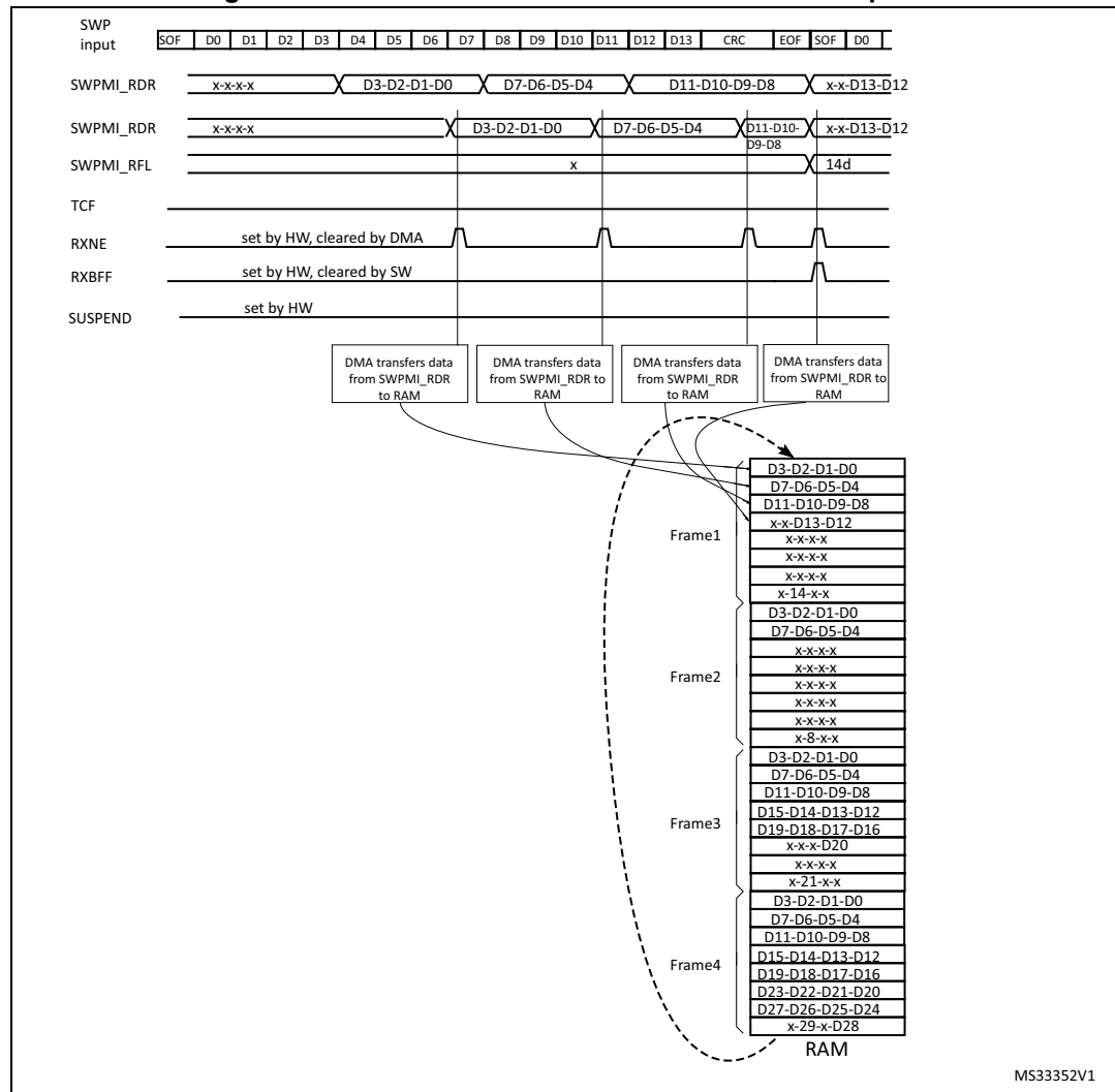
Figure 460. SWPMI Multi software buffer mode reception
