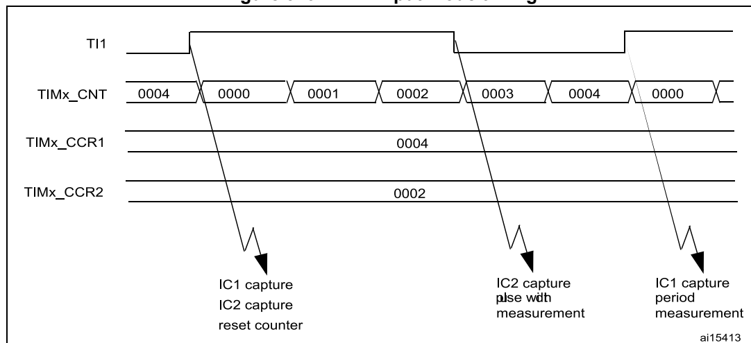
Figure 310. PWM input mode timing
