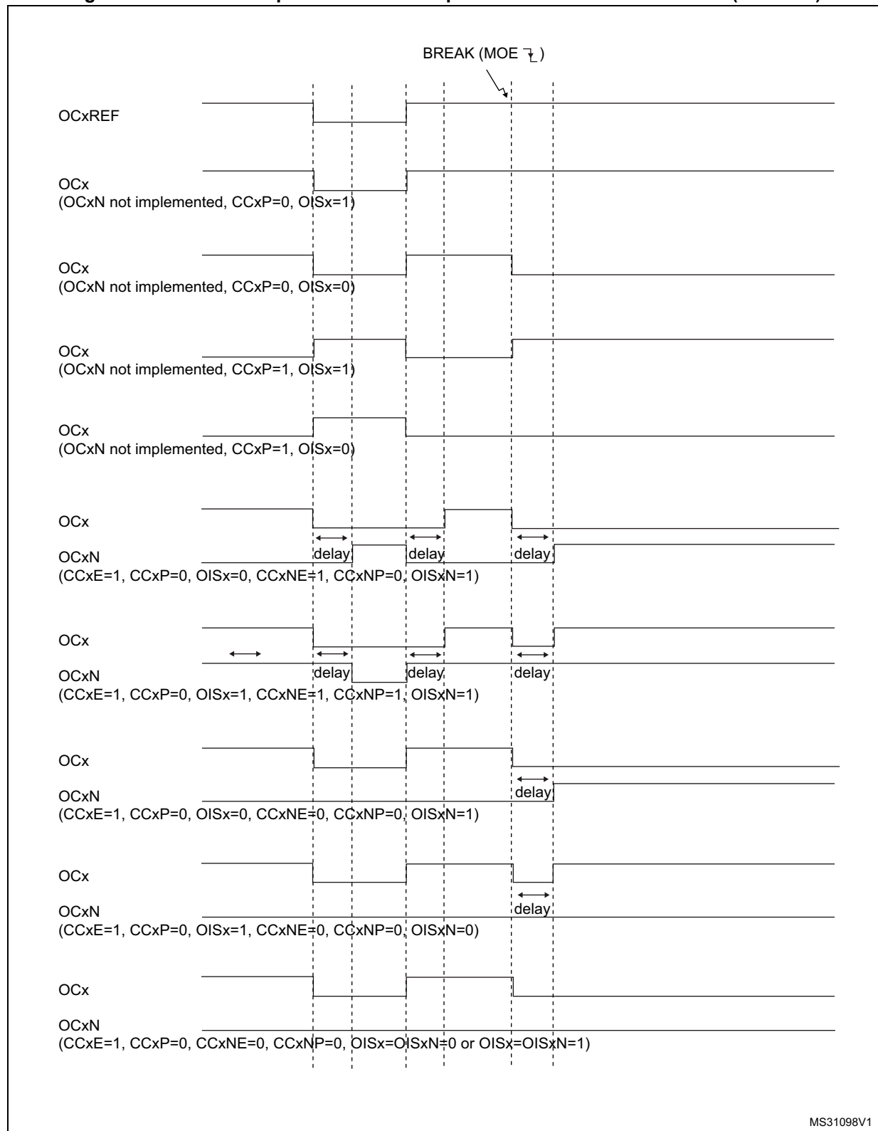
Figure 227. Various output behavior in response to a break event on BRK (OSSR = 1)
