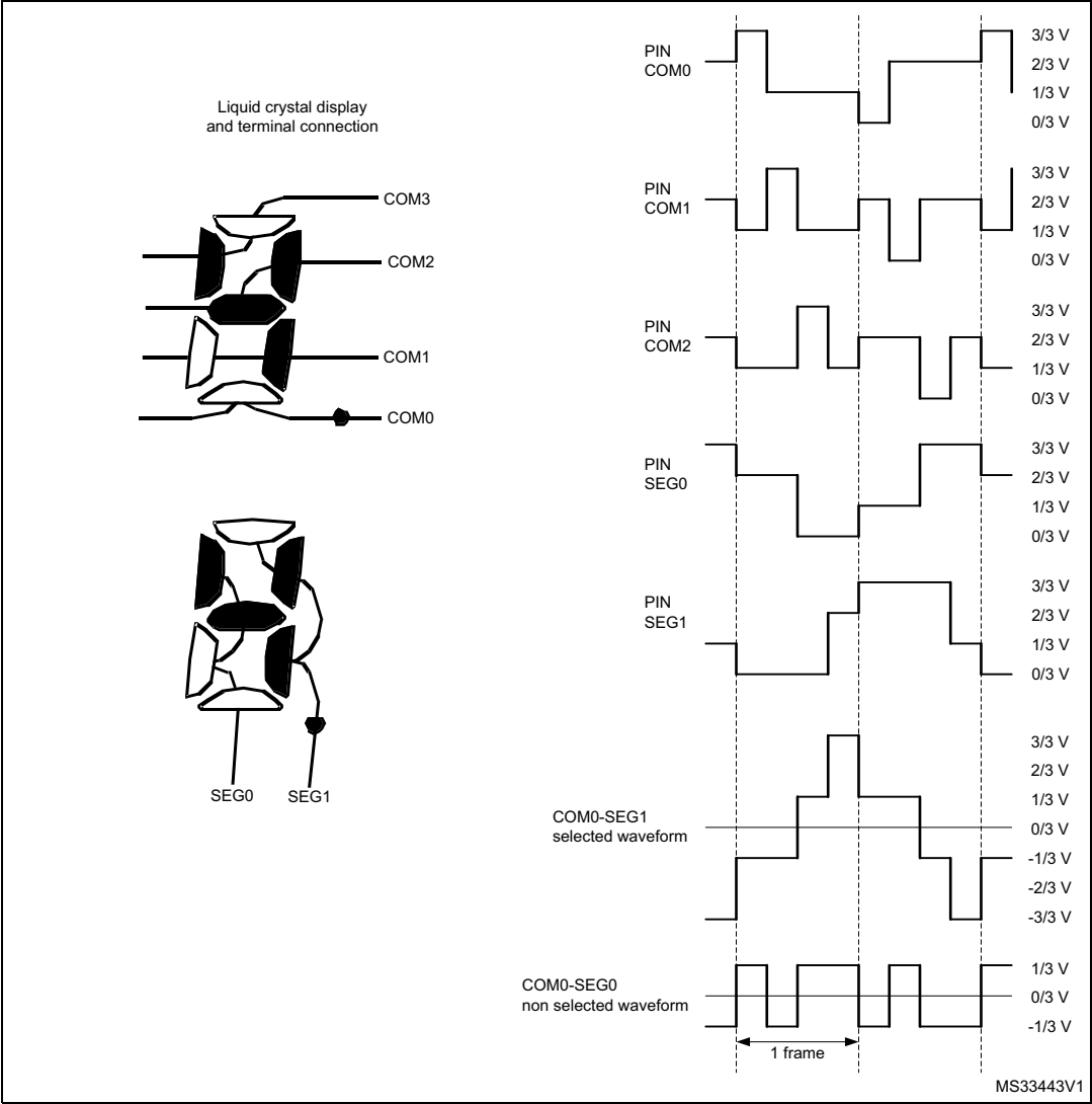
Figure 140. 1/4 duty, 1/3 bias
