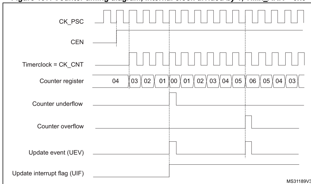
Figure 197. Counter timing diagram, internal clock divided by 1, TIMx_ARR = 0x6
