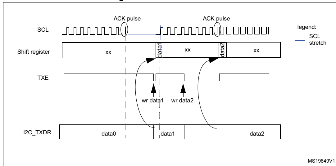
Figure 357. Data transmission
