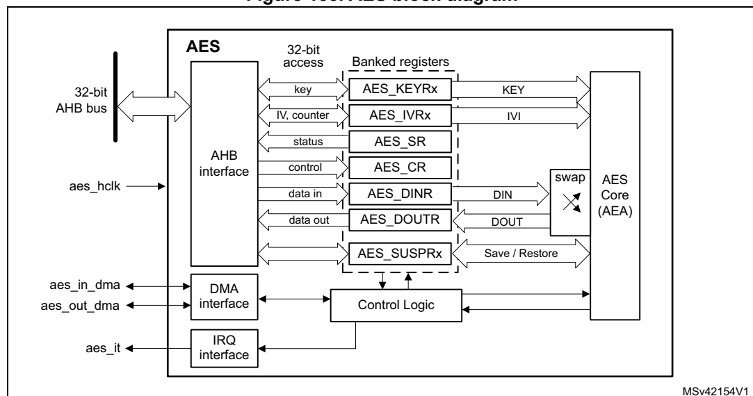
Figure 153. AES block diagram
