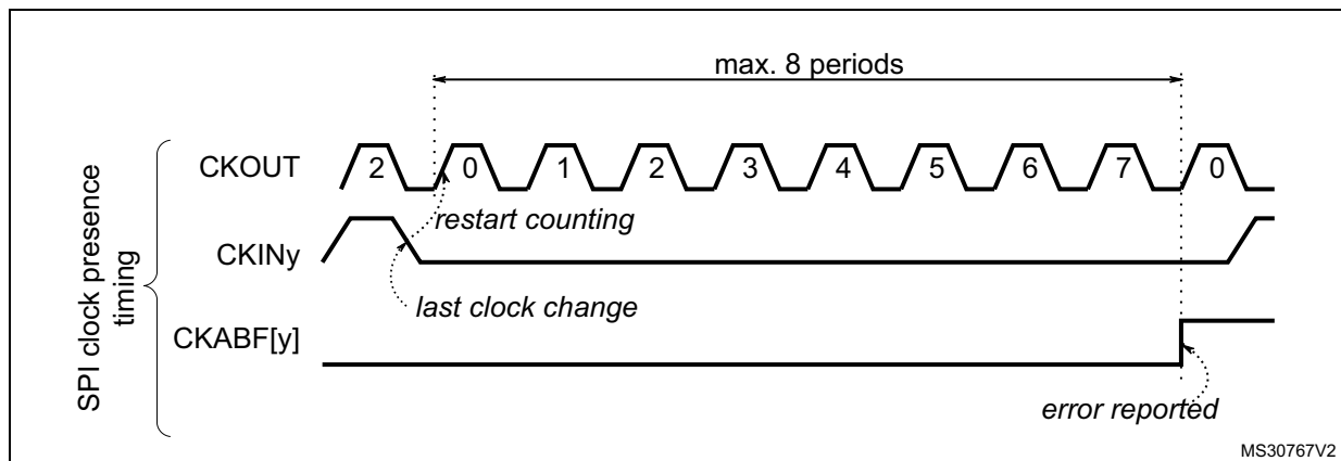
Figure 129. Clock absence timing diagram for SPI
