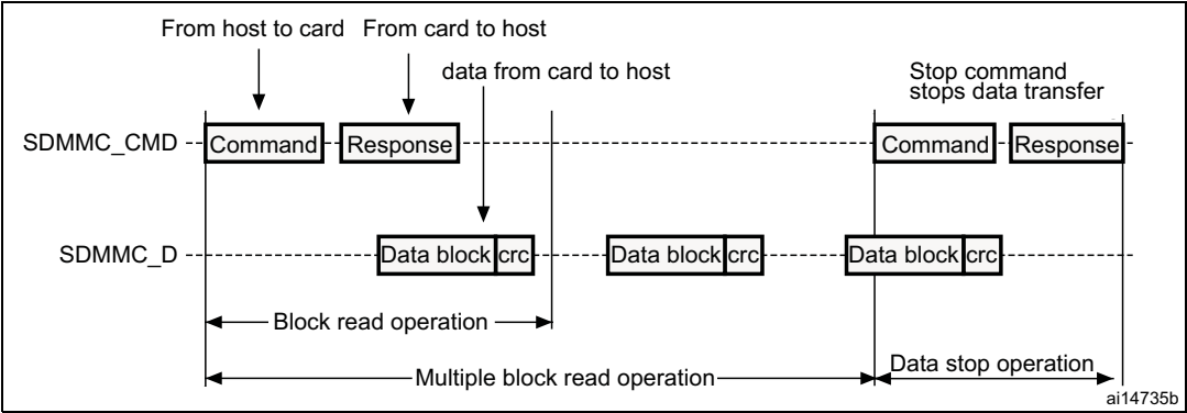
Figure 463. (Multiple) block read operation
