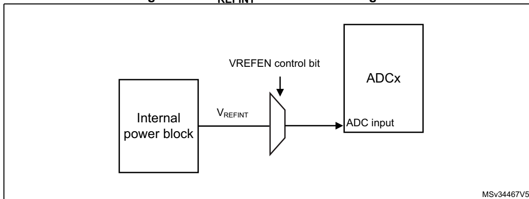
Figure 108. V_{REFINT} channel block diagram
