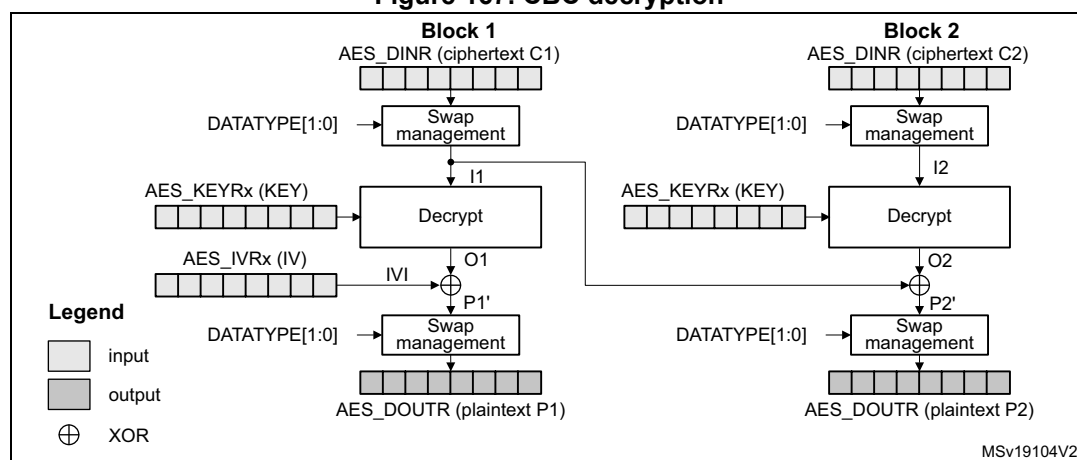
Figure 167. CBC decryption
