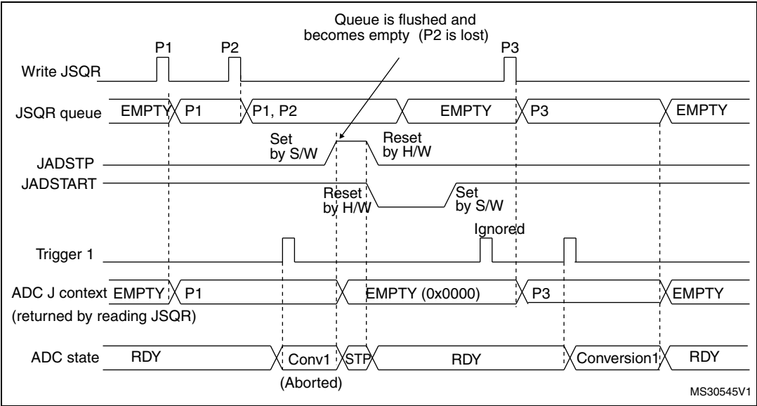
Figure 61. Flushing JSQR queue of context by setting JADSTP=1 (JQM=1)
