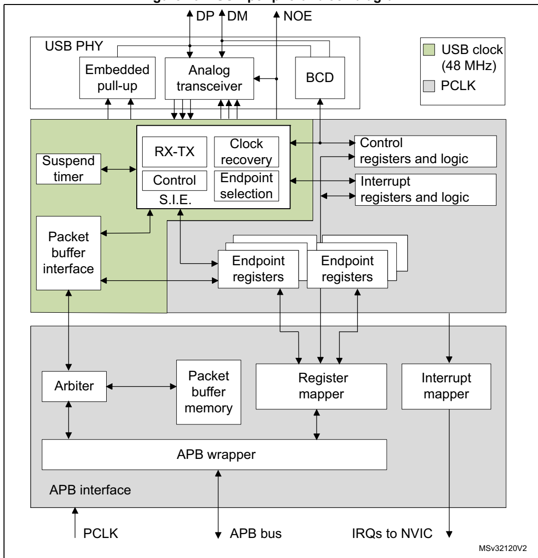
Figure 492. USB peripheral block diagram
