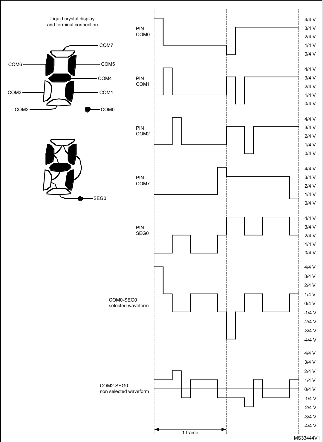
Figure 141. 1/8 duty, 1/4 bias
