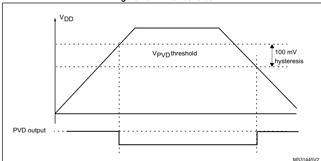
Figure 10. PVD thresholds
