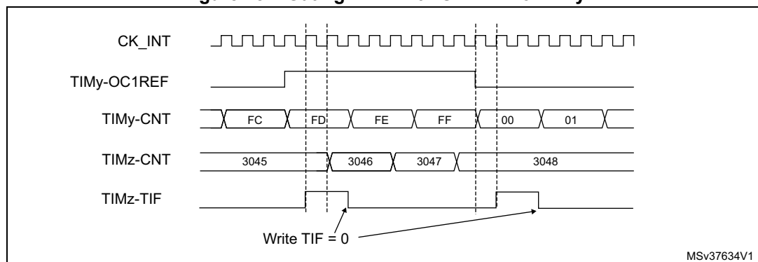
Figure 287. Gating TIMz with OC1REF of TIMy
