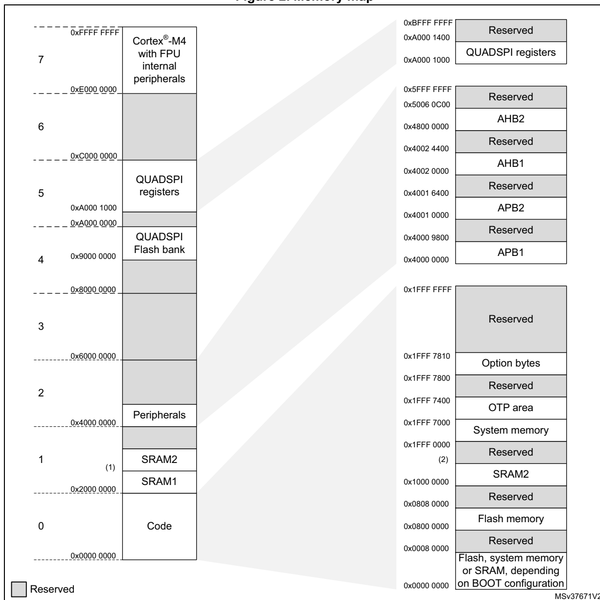
Figure 2. Memory map
