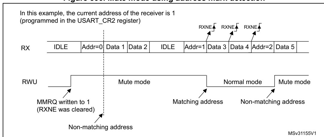
Figure 390. Mute mode using address mark detection
