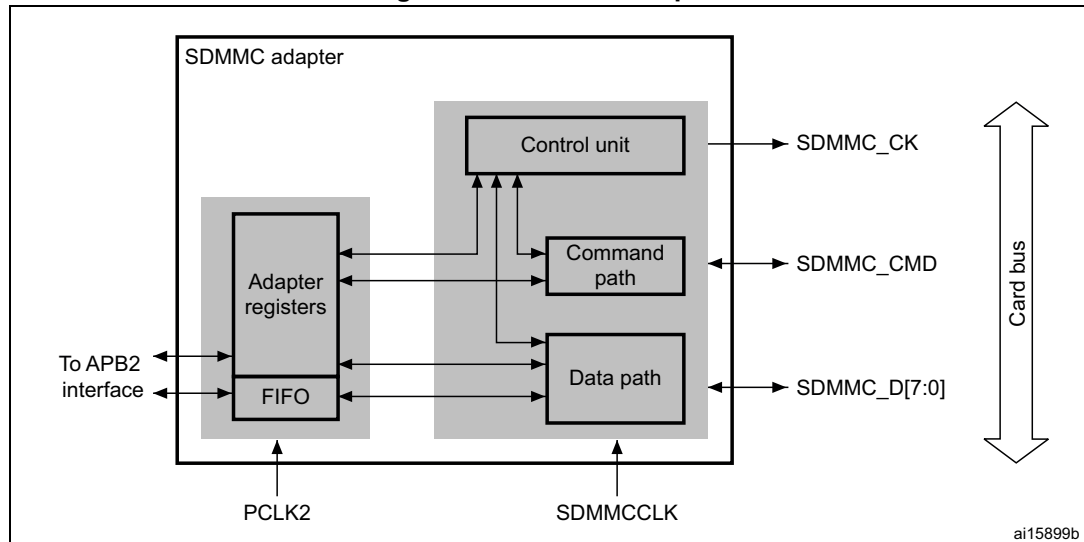
Figure 468. SDMMC adapter
