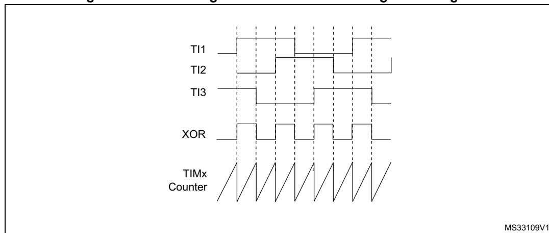
Figure 237. Measuring time interval between edges on 3 signals
