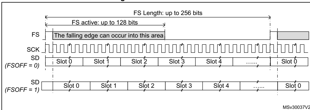
Figure 436. Audio frame
