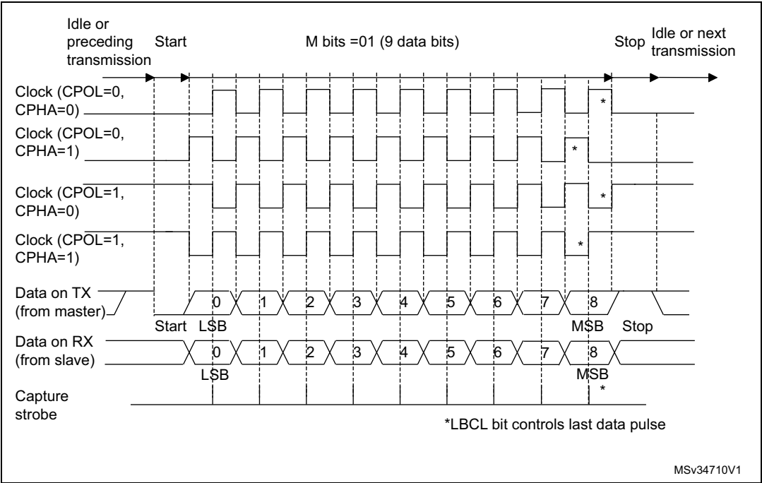
Figure 395. USART data clock timing diagram (M bits = 01)
