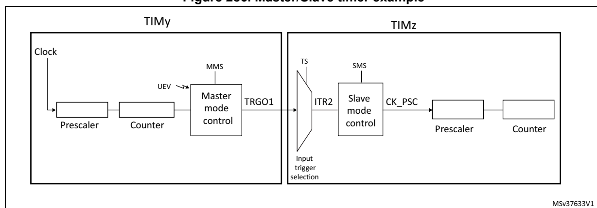
Figure 286. Master/Slave timer example
