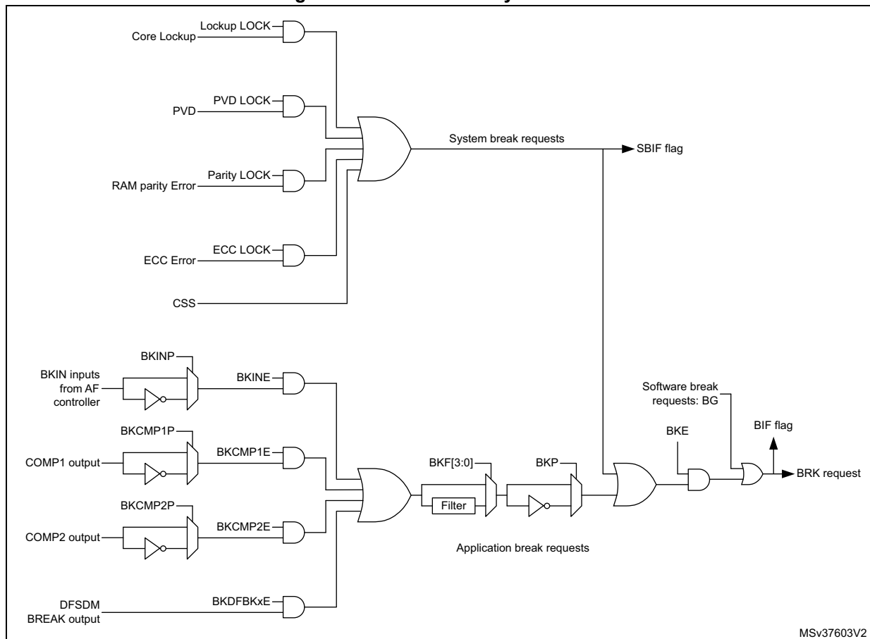
Figure 317. Break circuitry overview
