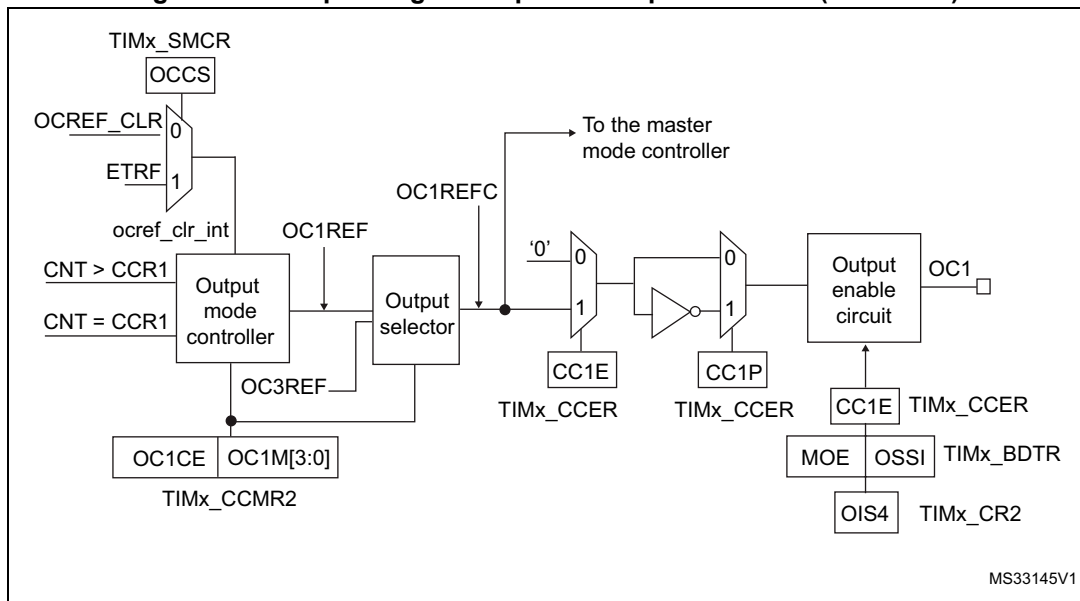
Figure 270. Output stage of Capture/Compare channel (channel 1)
