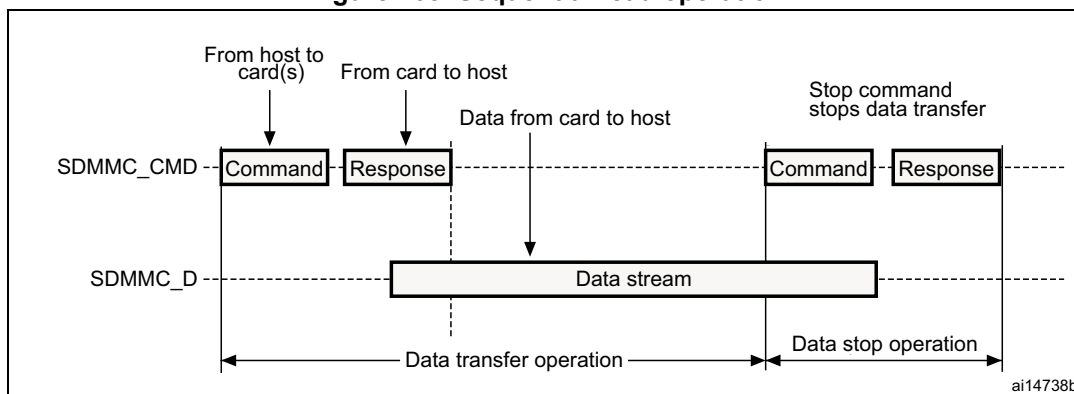
Figure 465. Sequential read operation
